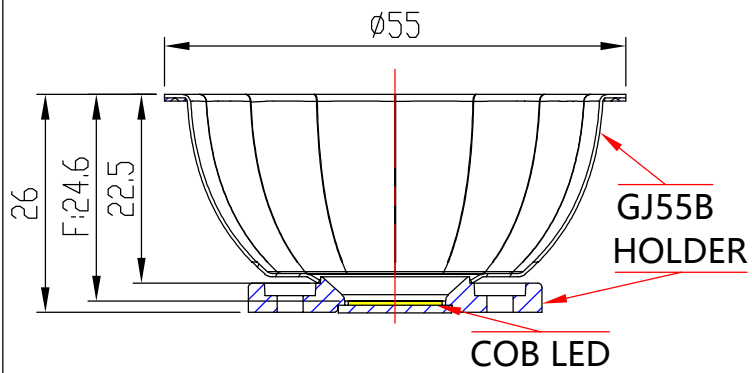
OPTICAL ASSEMBLY DIAGRAM
